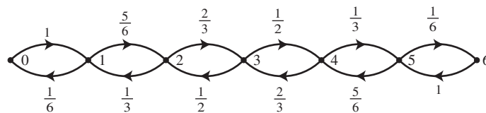
FIGURE 2 Transition diagram of the Ehrenfest urn model.
