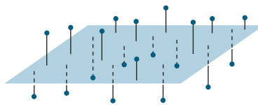
FIGURE 7 A least-squares plane.
