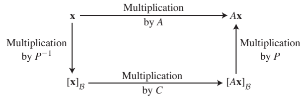
FIGURE 4 Similarity of two matrix representations: A = PCP^{-1} .
