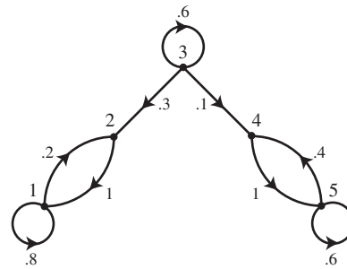
FIGURE 4 Transition diagram for Example 4.
